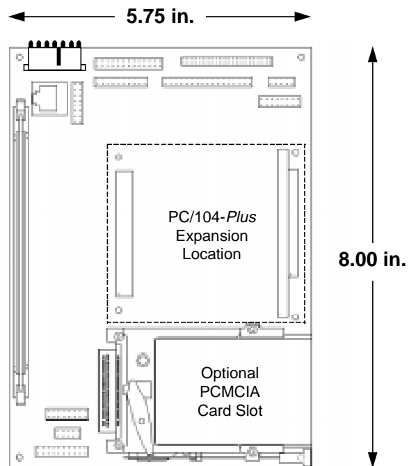
EBX Form-factor
